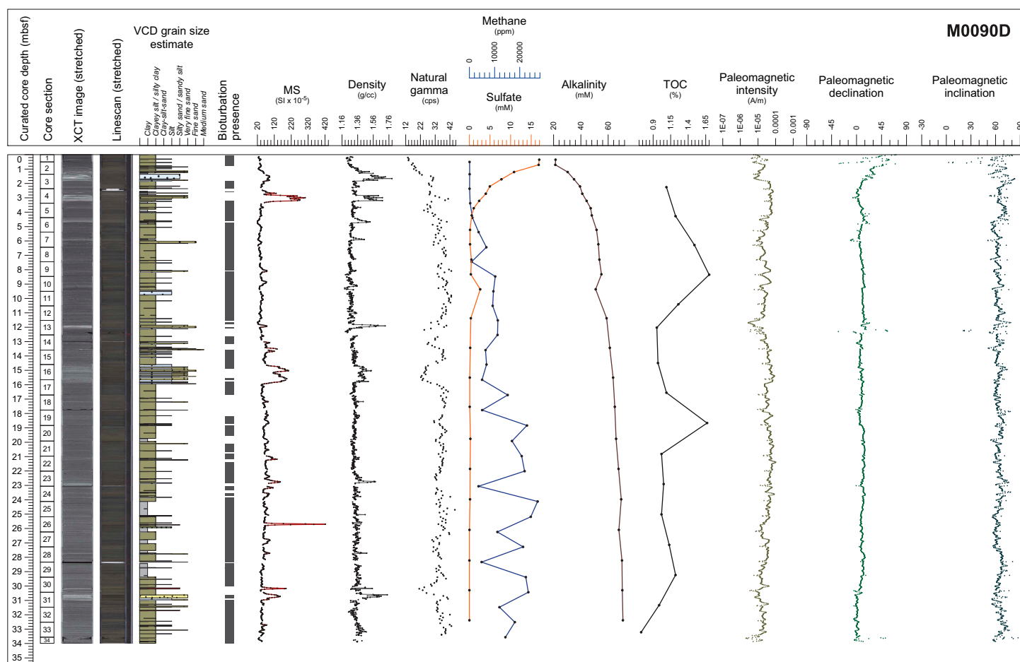
Figure F17. Composite Strater plot, Hole M0090D. For lithology legend, see Figure F9.
